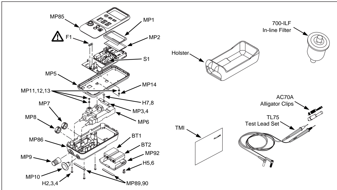
Figure 10. Replacement Parts
